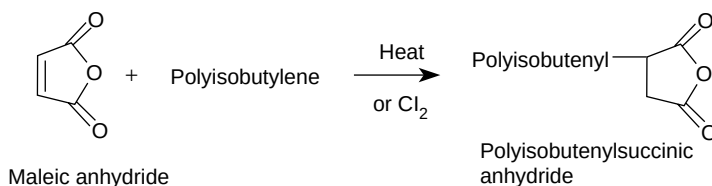
FIGURE 5.4 Alkenylsuccinic anhydride formation.
