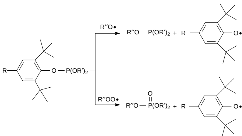
FIGURE 1.17 Alkoxy and peroxy scavenging mechanisms of phenyl phosphite.
