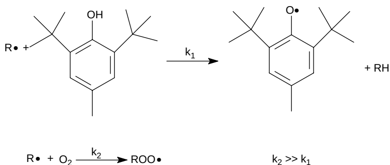
FIGURE 1.8 Reactivity of BHT with alkyl radical.
