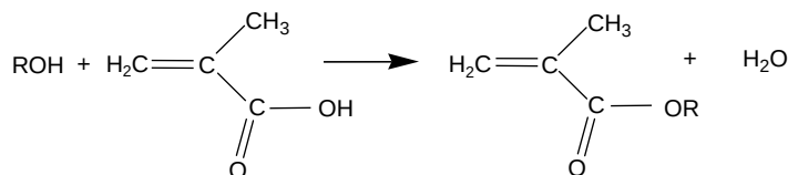
FIGURE 11.3 Direct esterification of methacrylic acid and alcohol.
