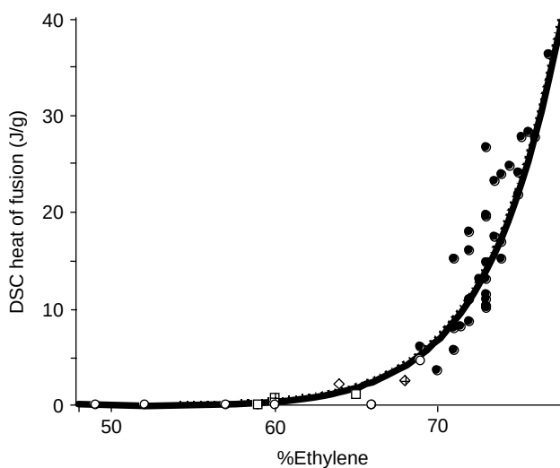
FIGURE 10.7 The effect of ethylene content (wt%) on crystallinity as measured by differential scanning calorimetry (DSC) for a range of experimental EPDM copolymers.
