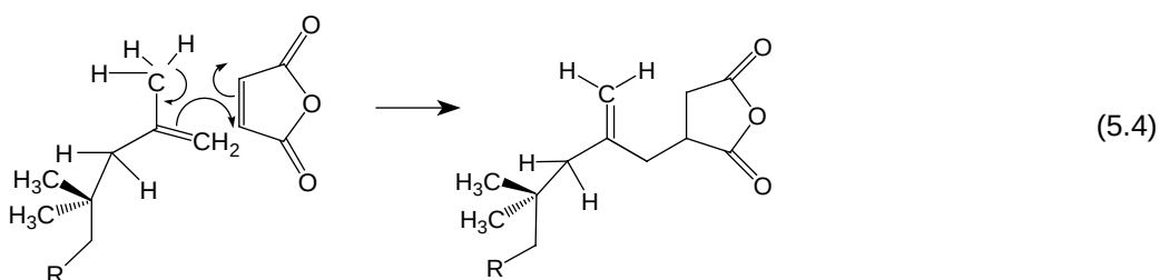
FIGURE 5.6 Mechanism of alkenylsuccinic anhydride formation.
