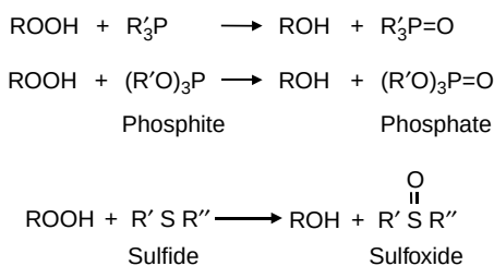
FIGURE 19.29 Mechanism of S- and P-containing antioxidants.
