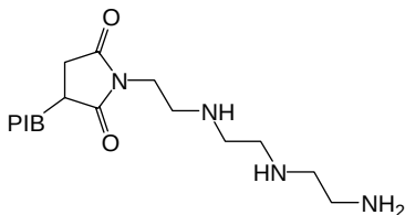
FIGURE 19.11 Example of monosuccinimide from triethylenetetramine (TETA).
