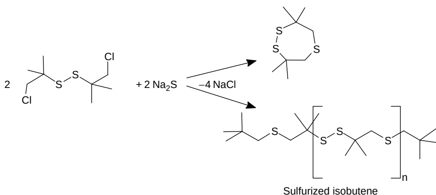
FIGURE 9.9 Dechlorination reaction.
