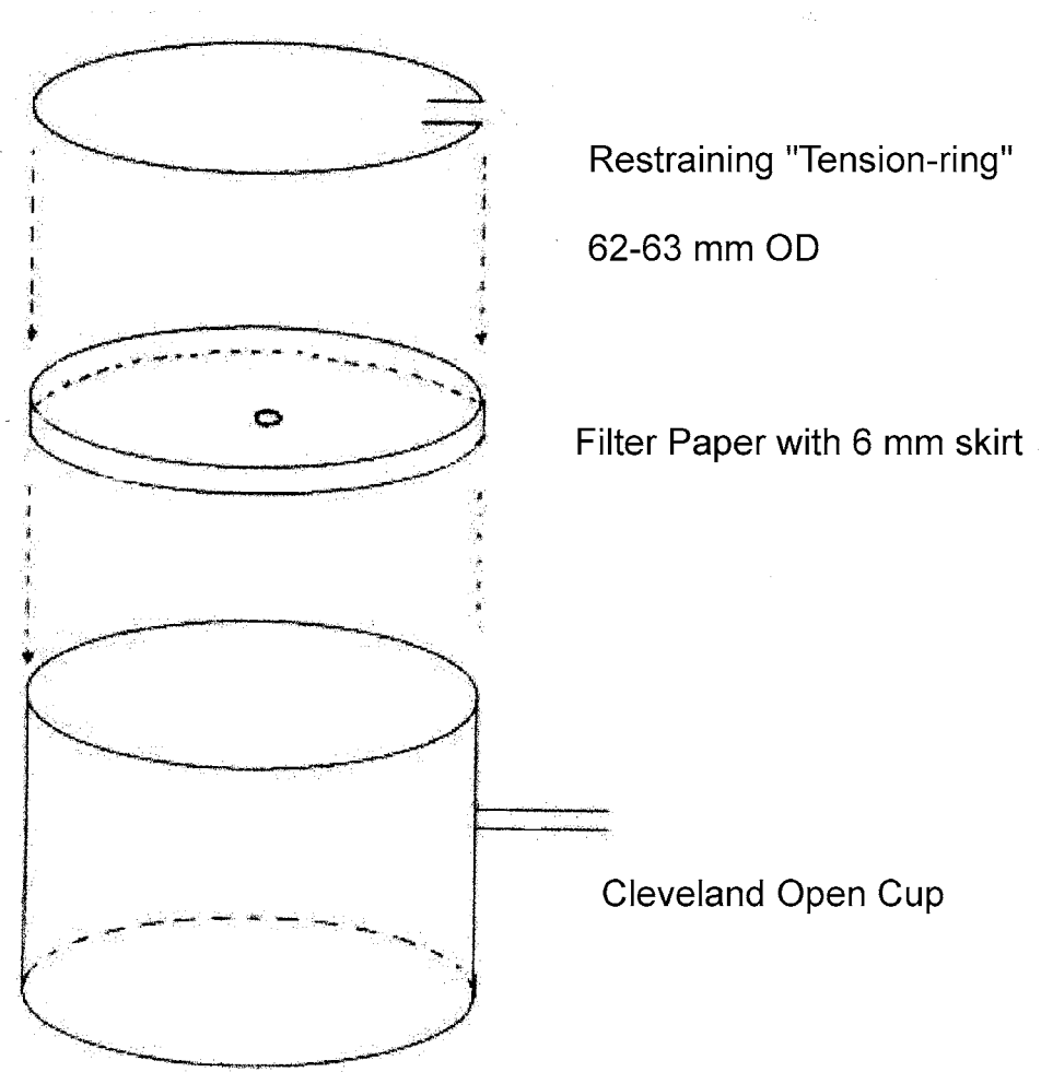
FIG. X1.1 Technique to Prevent Surface Skin Formation When Testing Flash Point of Asphalts by Test Method D92
